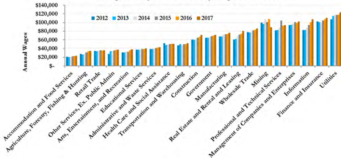
Orange County Annual Industry Wages, 2012-2017
