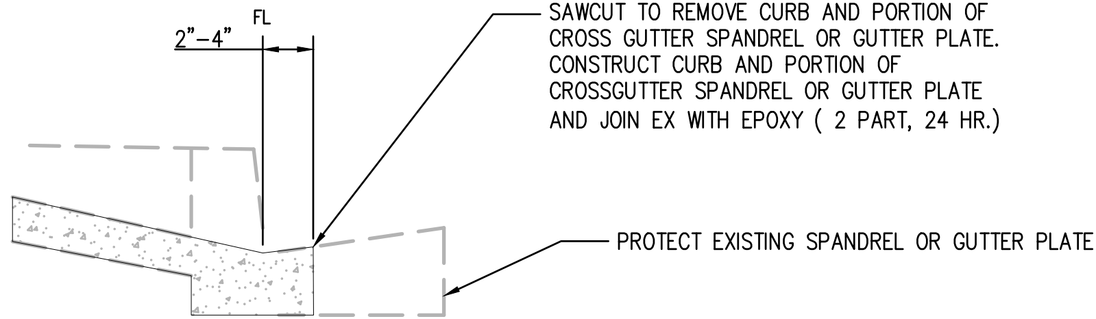
SAWCUT DETAIL "2" AT SPANDREL OR CROSS GUTTER N.T.S.
